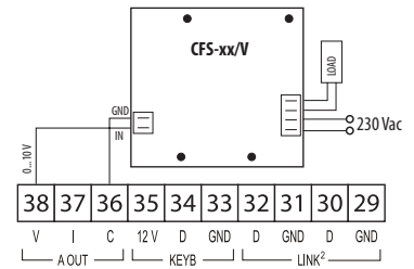
FH with CFS-xx/V on 0...10 V output
